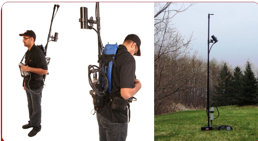
Optically pumped Potassium Magnetometer (GSMP-35 v8.0) with ruggedized console, backpack for electronics, light weight sensors and cables.
